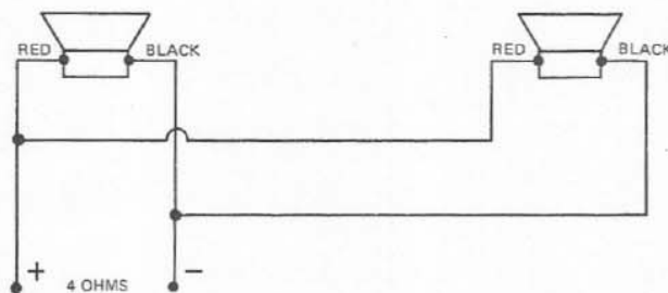
FIGURE 4 — Connection of 2 SRO/15L Speakers in Parallel
